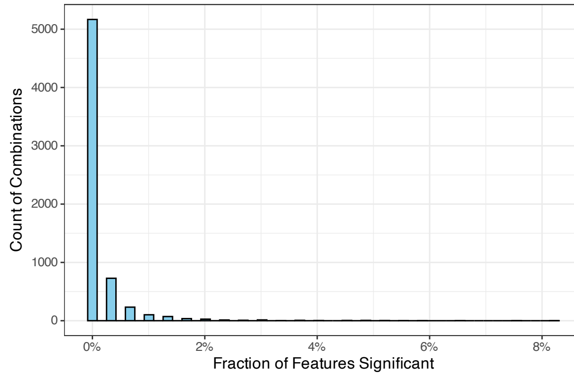
Distribution of Fraction of Significant Features
