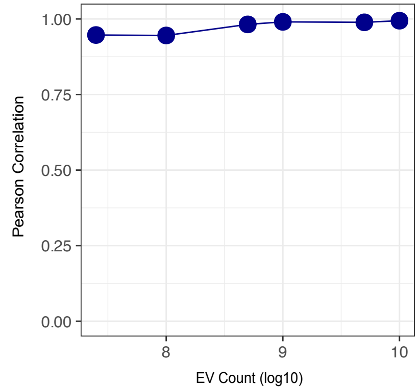
Reproducibility of miRNA Profiles Between Replicates
