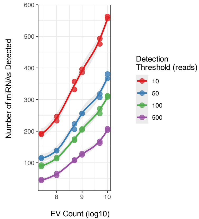
miRNA Detection Sensitivity by EV Input
