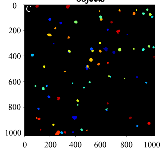
IdentifyPrimaryObjects objects
